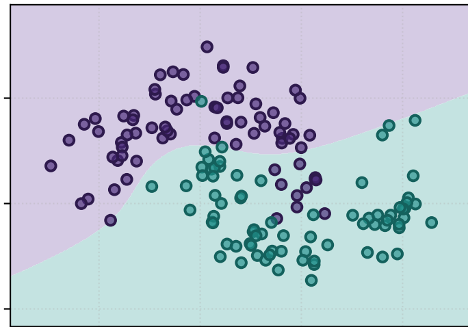
(b) Polynomial ( d=3 ) — acc. test = 0.92
